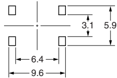
PCB Pad (Top View) (One-side PCB t= 1.6)
